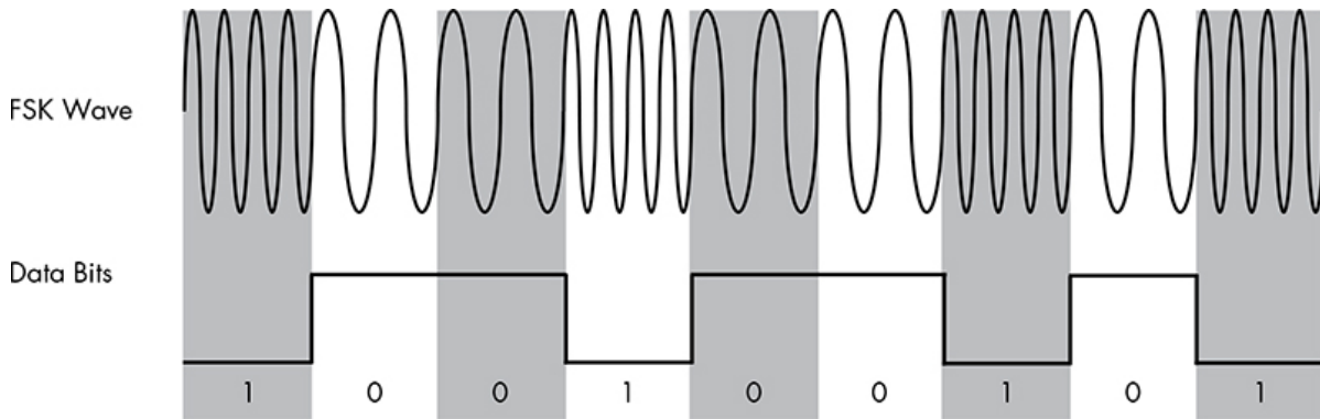
Figure 12-2: FSK modulation
