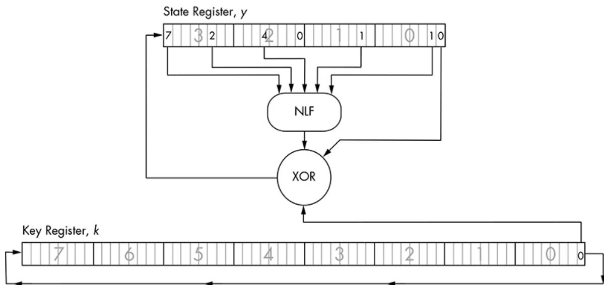
Figure 12-8: Keeloq algorithm
