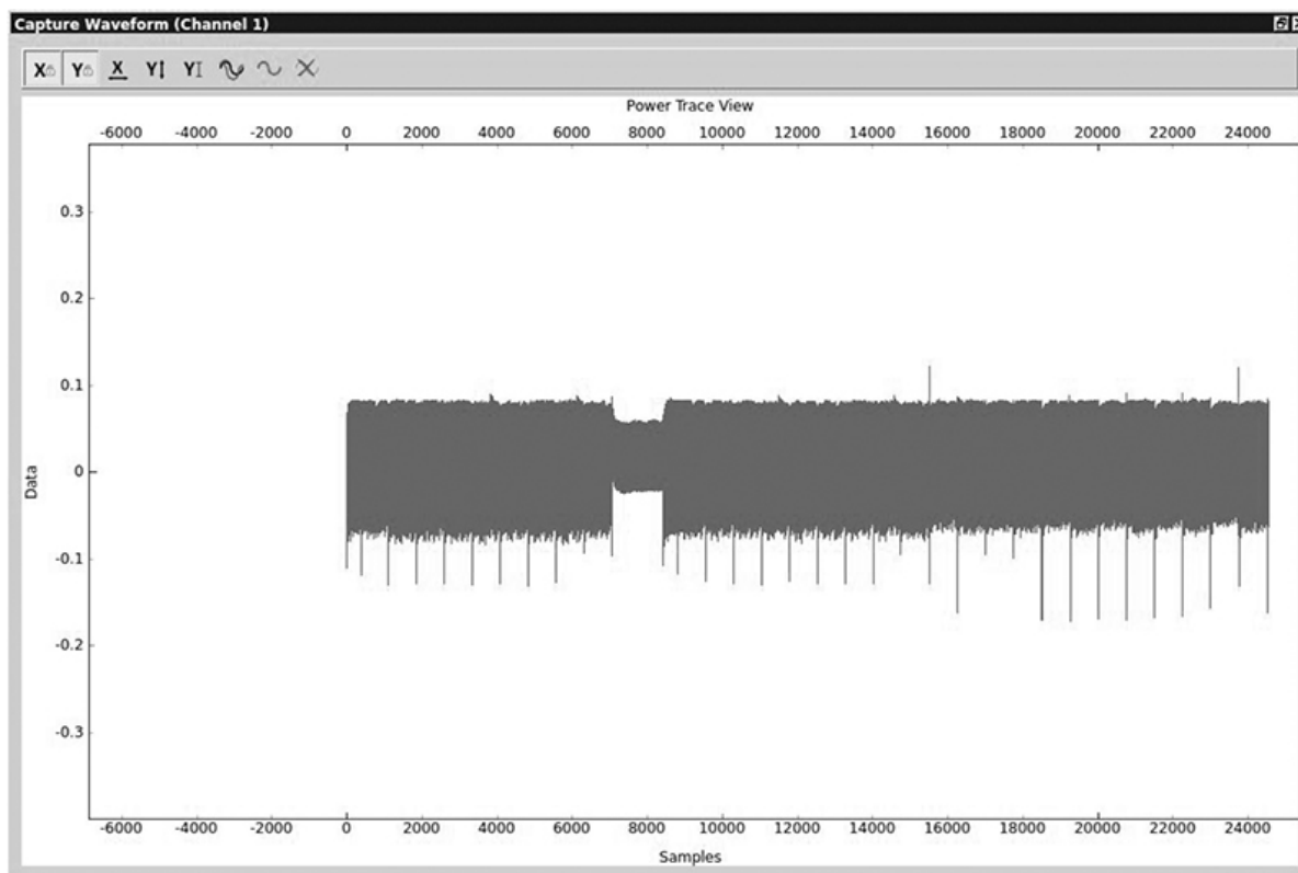
Figure 8-16: Power trace of a valid password
