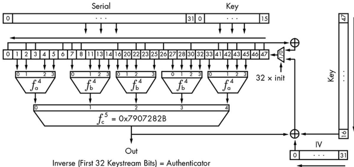
Figure 12-7: Hitag 2 cipher
