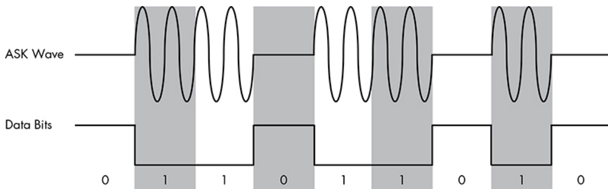
Figure 12-1: ASK modulation
